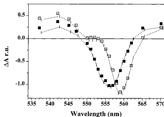
FIGURE 4: Spectra of c559 and c556 oxidation computed from the kinetic data. The spectra were computed by solving the following equations: (1) \Delta A^f(\lambda) = \alpha(\Delta \epsilon_P - \Delta \epsilon_{c559}) ; (2) \Delta A^s(\lambda) = (1 - \alpha)(\Delta \epsilon_P - \Delta \epsilon_{c556}) + \alpha(\Delta \epsilon_{c559} - \Delta \epsilon_{c556}) , where \Delta A^f(\lambda) and \Delta A^s(\lambda) stand for the amplitude of the submicrosecond and microsecond phases at wavelength \lambda , respectively; \alpha stands for the relative amplitude of the submicrosecond phase; and \Delta \epsilon_P , \Delta \epsilon_{c559} , and \Delta \epsilon_{c556} are the absorbance changes due to P , c559 , and c556 oxidation, respectively. Closed squares, spectrum of c559 oxidation; open squares, spectrum of c556 oxidation, both in the presence of the permanent \Delta \tilde{\mu}_H . Spectra obtained in the absence of the permanent \Delta \tilde{\mu}_H are shown by bars and dotted lines.
